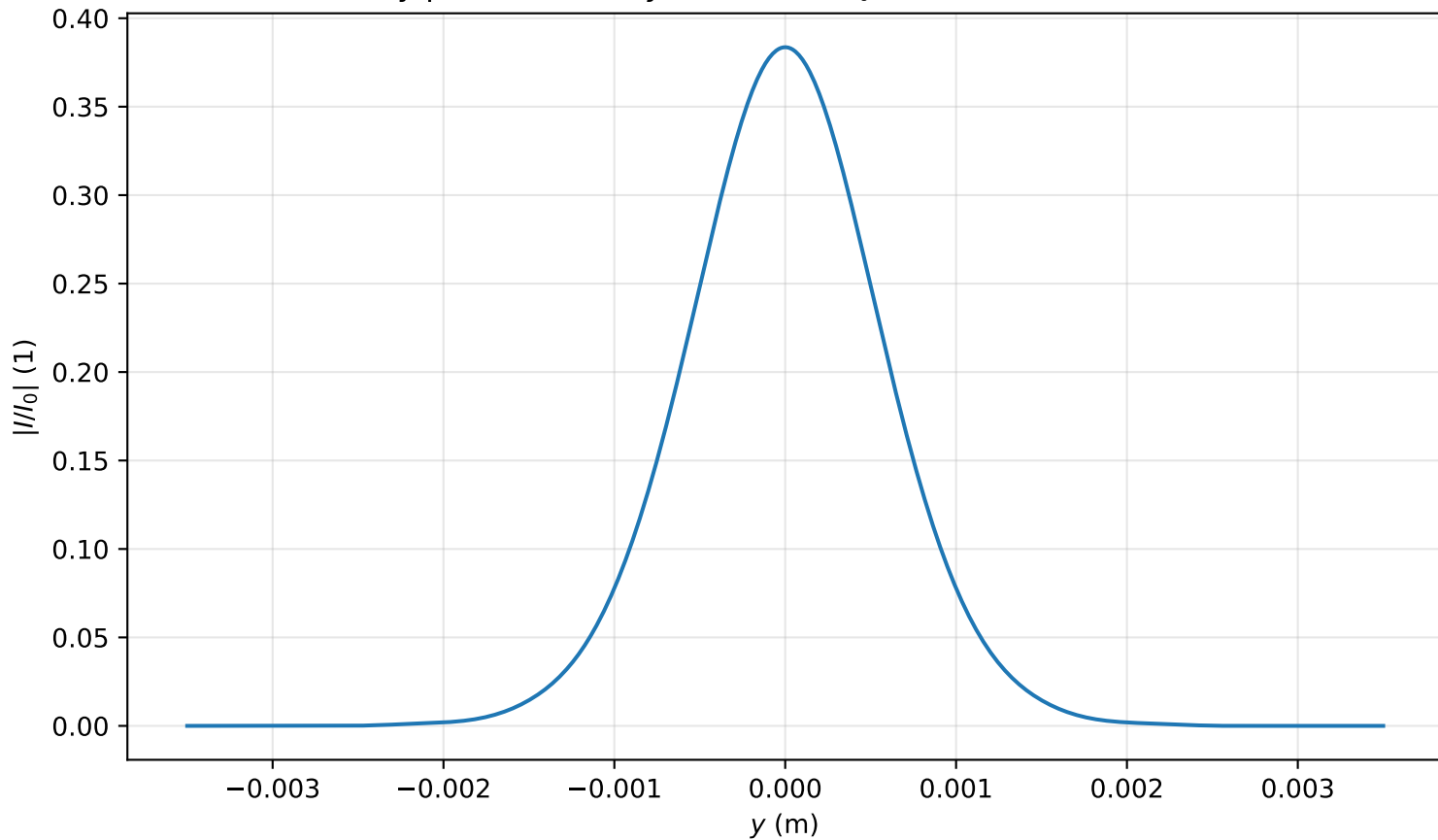
Intensity profile I(x=0, y, z=3.582)/I_0 , P_{in}=0.4P_{cr} , artificial time
